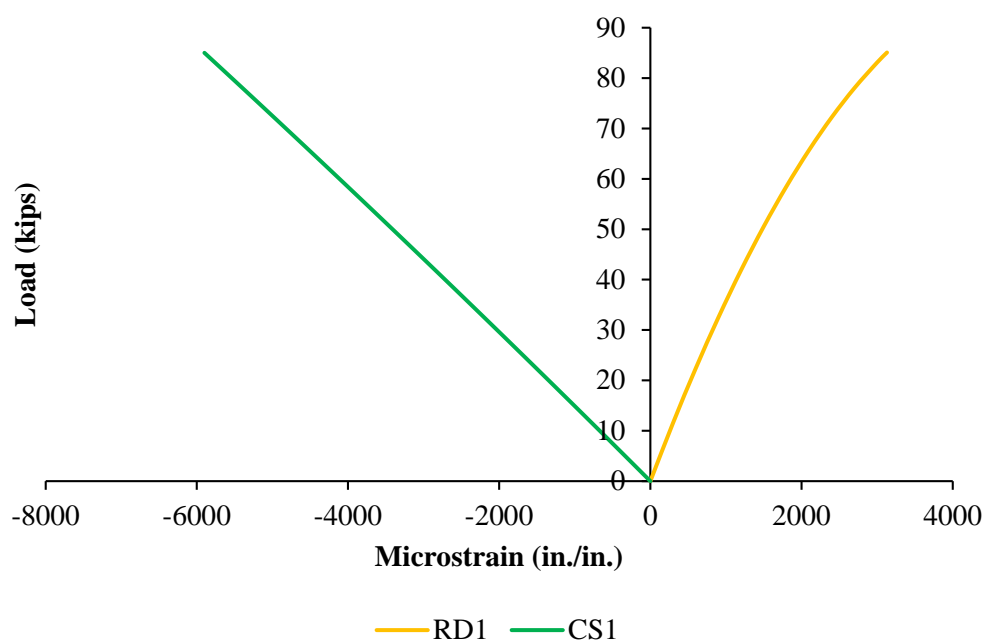
Figure B. 25 Load versus strain for specimen B-1-C-C-N
