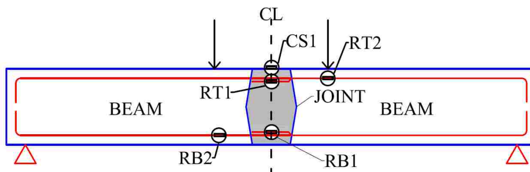
Figure B. 1 Location of strain gages in Phase one
