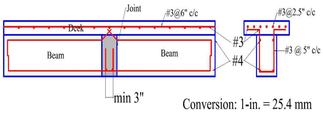
Figure 3.11 Specimen with reinforcement layout (with MoDOT detail) and cross-section
