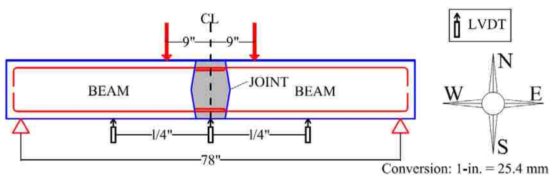
Figure A. 1 Test setup used
