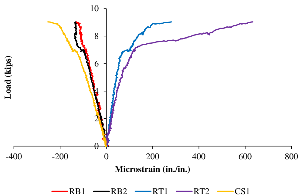
Figure B. 6 Load versus strain for specimen B-4-C-N-A
